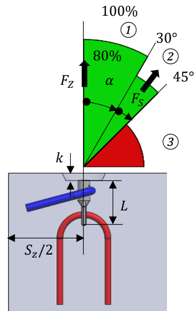
Axial & Diagonal pull lifting
