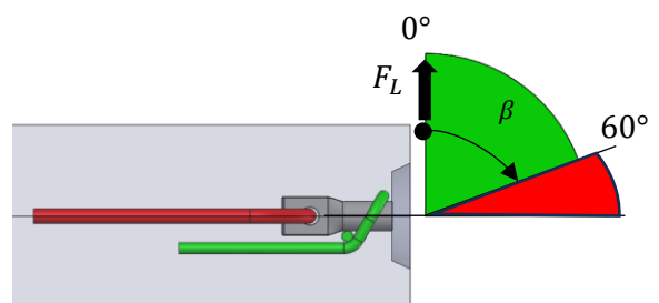
Tilt-up and turning lifting
